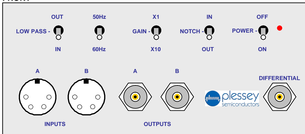
Control and Interface box front panel
