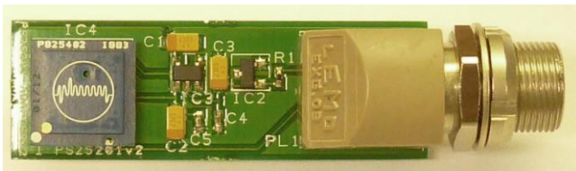
Figure 1: PS25014A2 single channel board carrying a single PS25402 sensor
