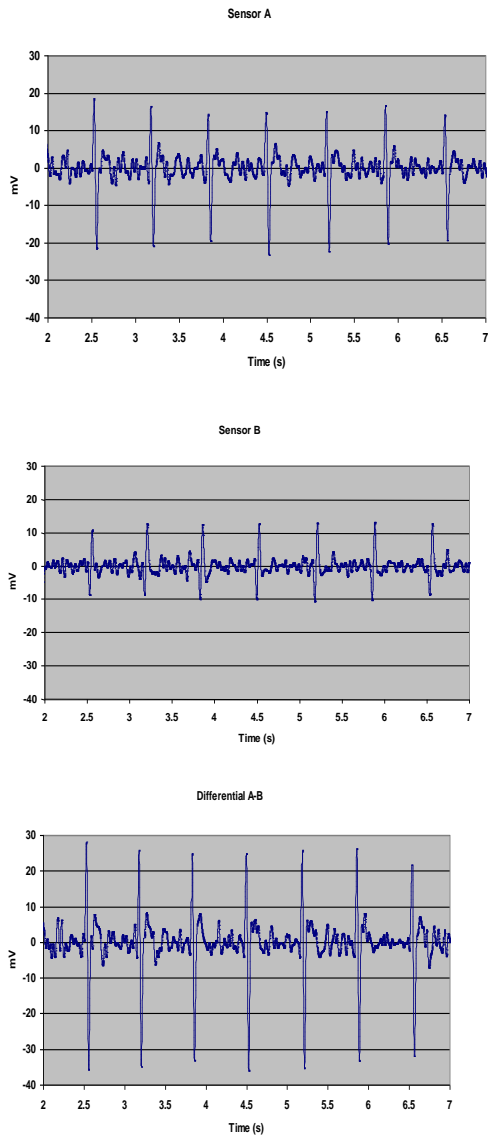
Figure 3 – ECG signals from sensors mounted in a sports armband on the left upper arm from a stationary subject. The graphs show the individual sensor outputs and the differential output, as labelled
