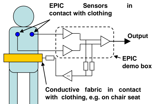
Basic configuration for non-contact ECG measurement including capacitively-coupled DRL" circuit.
