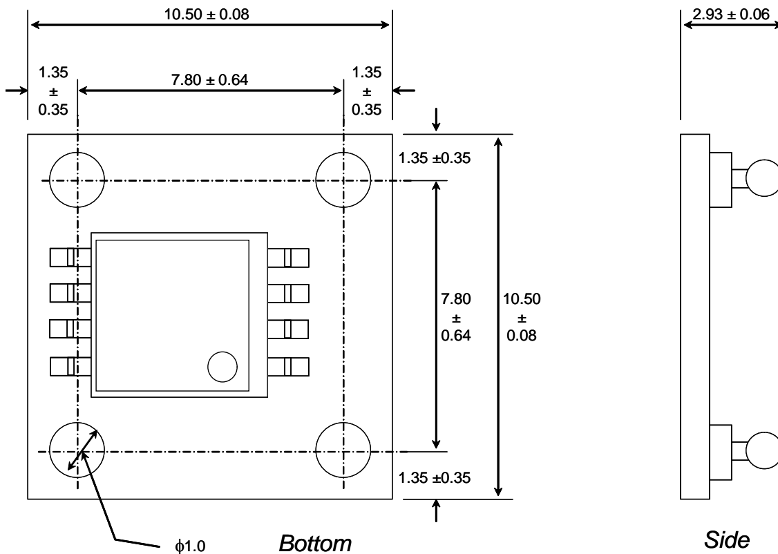
Mechanical Drawing (all dimensions are nominal and in mm)
