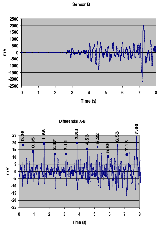
Figure 7 – ECG signals from sensors mounted in a sports armband on the left upper arm of a moving subject. The subject began walking after 2.5 seconds, as shown by the increase in signal amplitude on the individual sensors. Note that the y-axis scale is 100 times smaller for the differential trace (bottom) as the large common mode signals are rejected by the differential amplifier. The times corresponding to the QRS part of the ECG signal are shown on the differential trace.
